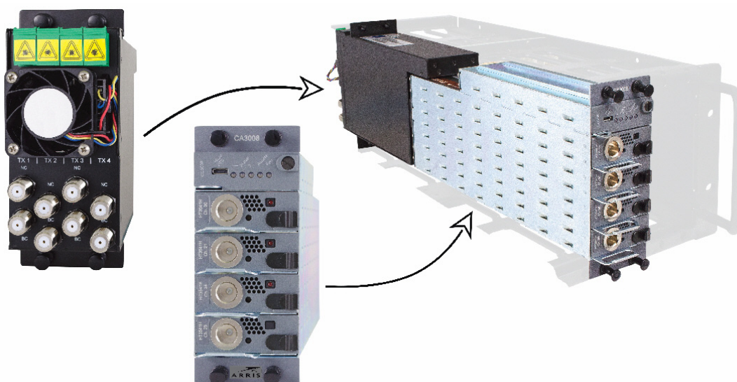
HT3300H Series Quad-Stack and CC3008 Communications Module joined with a BD31A4 Multiplexing Back Plate
